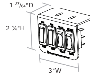
LCS653-013 switch panel
