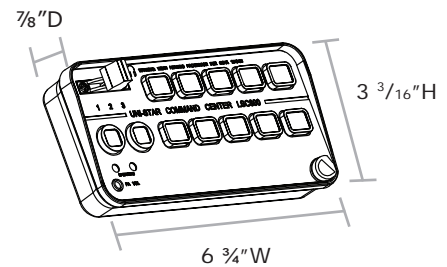
Flangeless Mount
